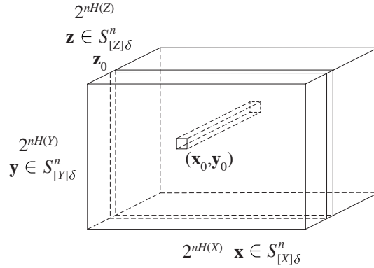
Fig. 6.3. A three-dimensional strong joint typicality array.
